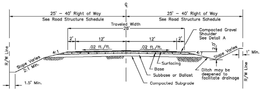
TYPICAL RURAL ROAD SECTION N.T.S.
